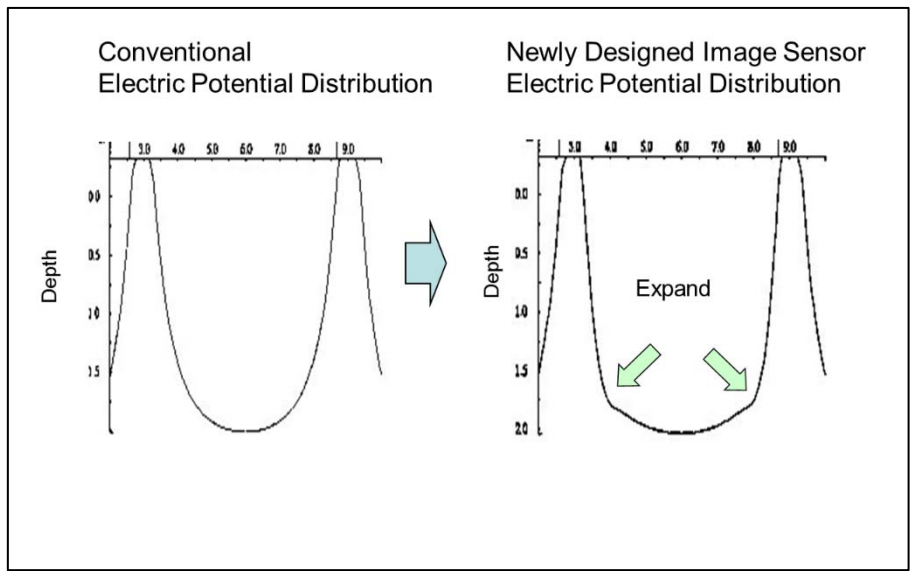
Fig. 3-1-1 High capacity Photodiodes
