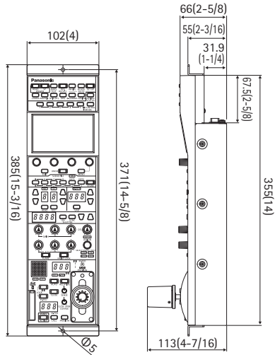
■ AK-HRP1000GJ
