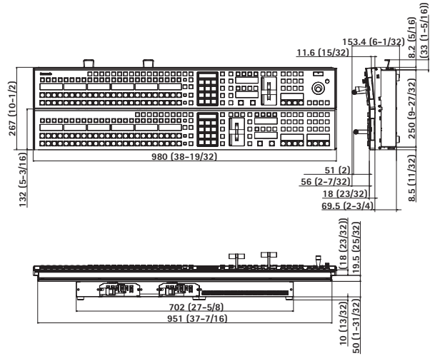
Control Panel AV-HS60C2P/AV-HS60C2E
